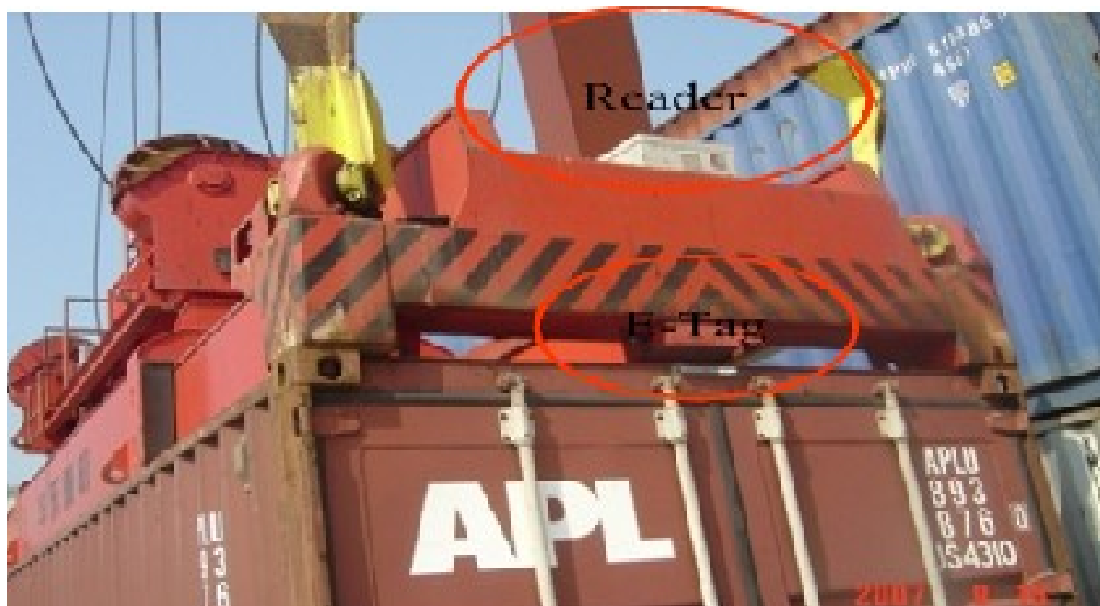
Figure 6 Reader installed on the gantry crane and the E-tag on the container
